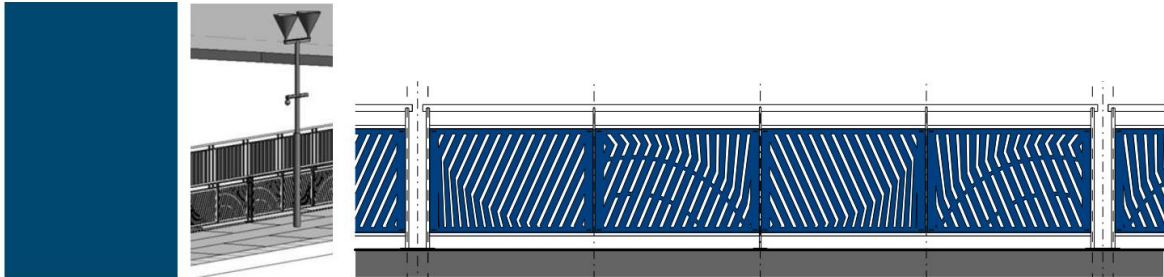
STATION METAL RAILING INFILL PANEL - Blueprint SW4056
